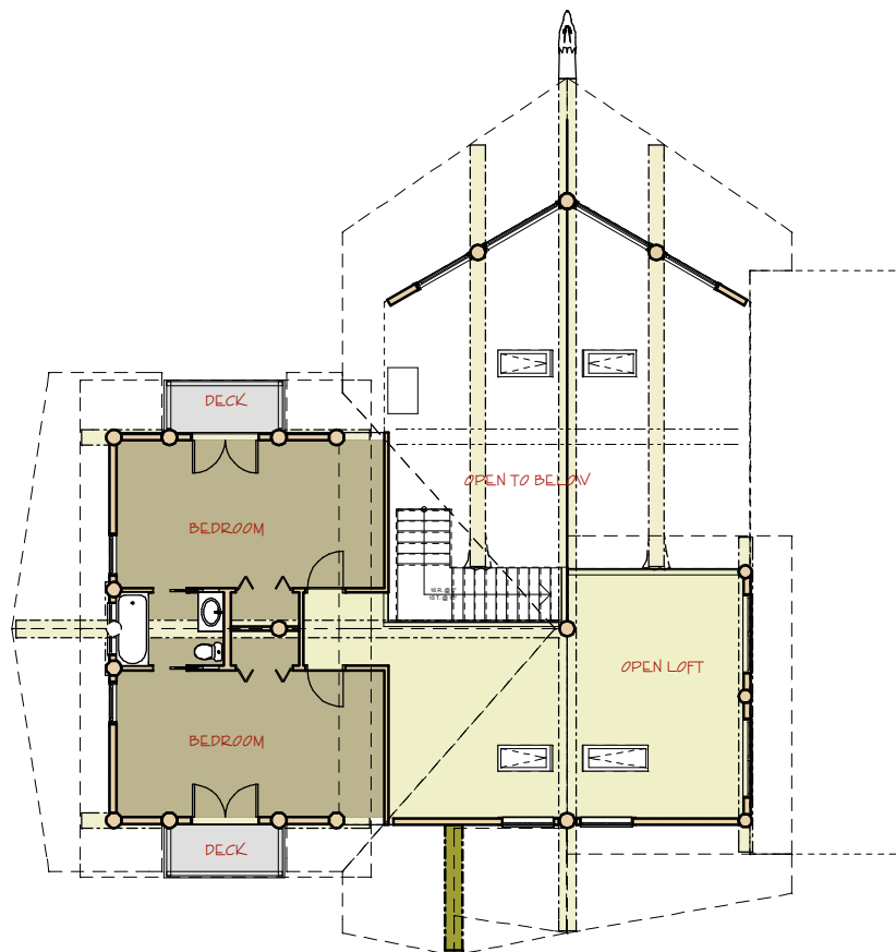
LOFT FLOOR PLAN
